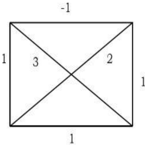
Given graph
